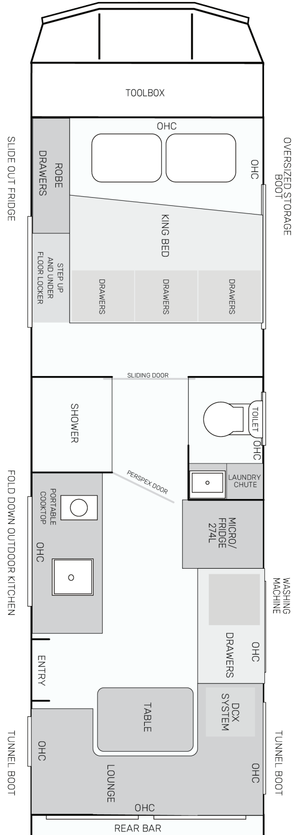
TOOLBOX LAYOUT (OPTIONAL UPGRADE) THE VAN WILL BE 350MM LONGER WITH THE TOOLBOX
